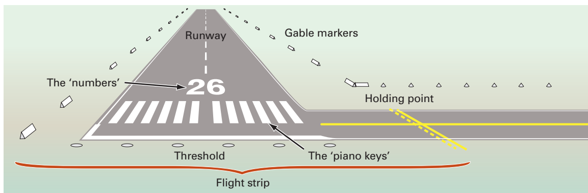
Figure 5-7 Runway and associated boundaries.
