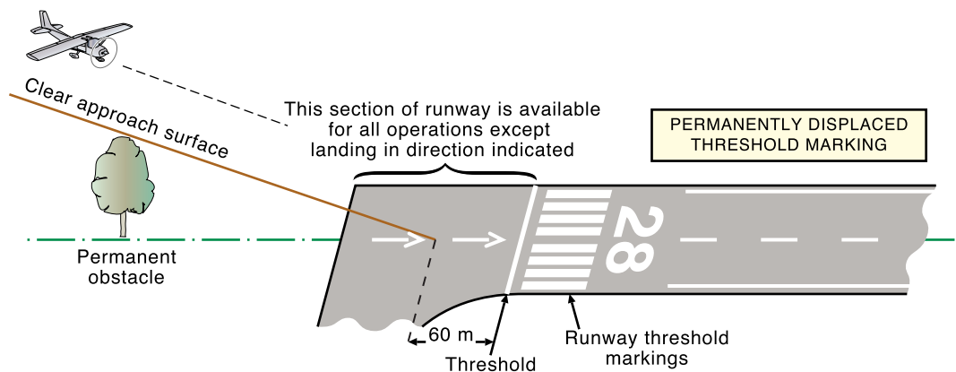
Figure 5-8 Permanently displaced threshold marking.
